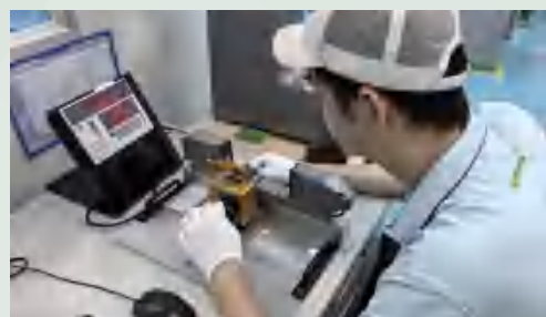
激光测径仪 Laser caliper
